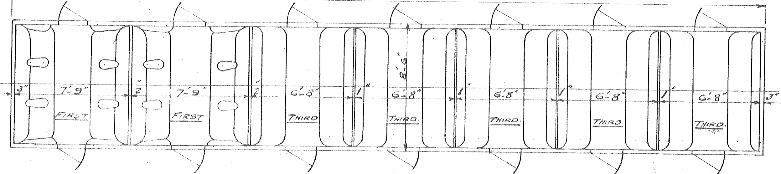
BOGIE COMPOSITE CARRIAGE (C.L.G.)
